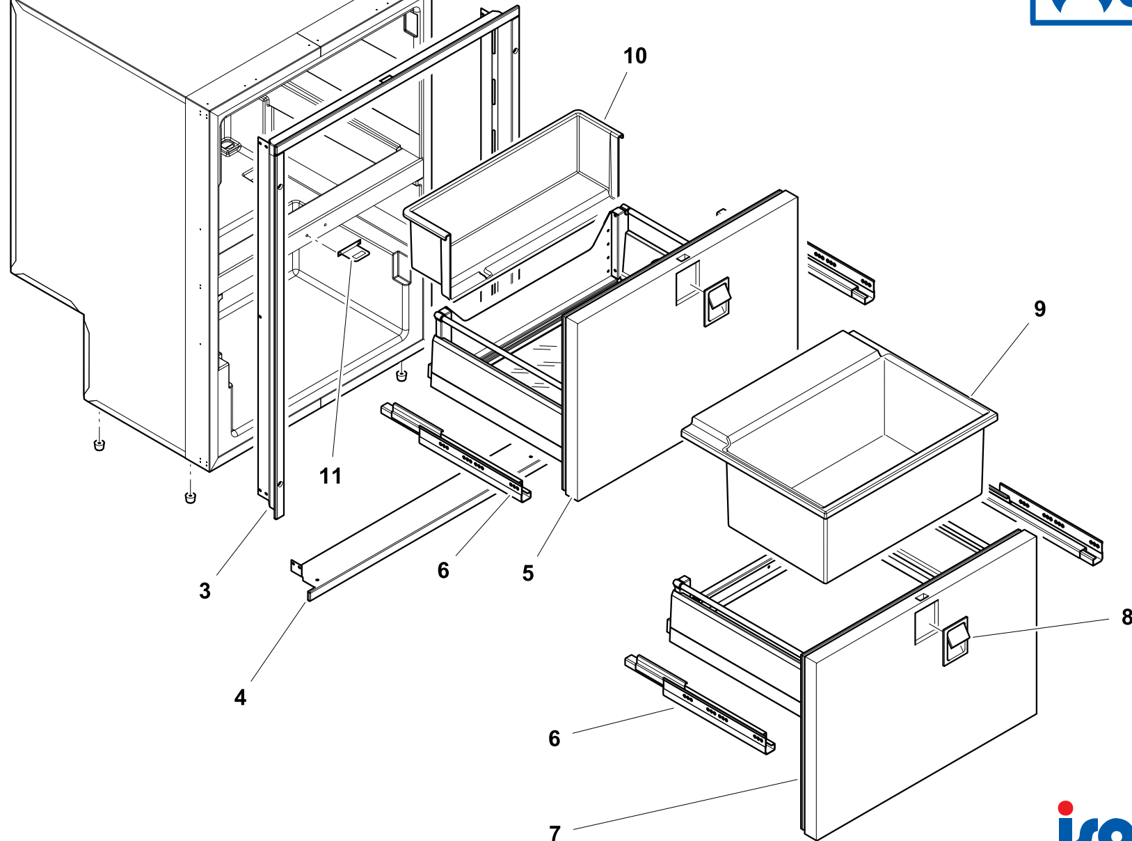
DR 160 Frigo-Freezer - CABINET
