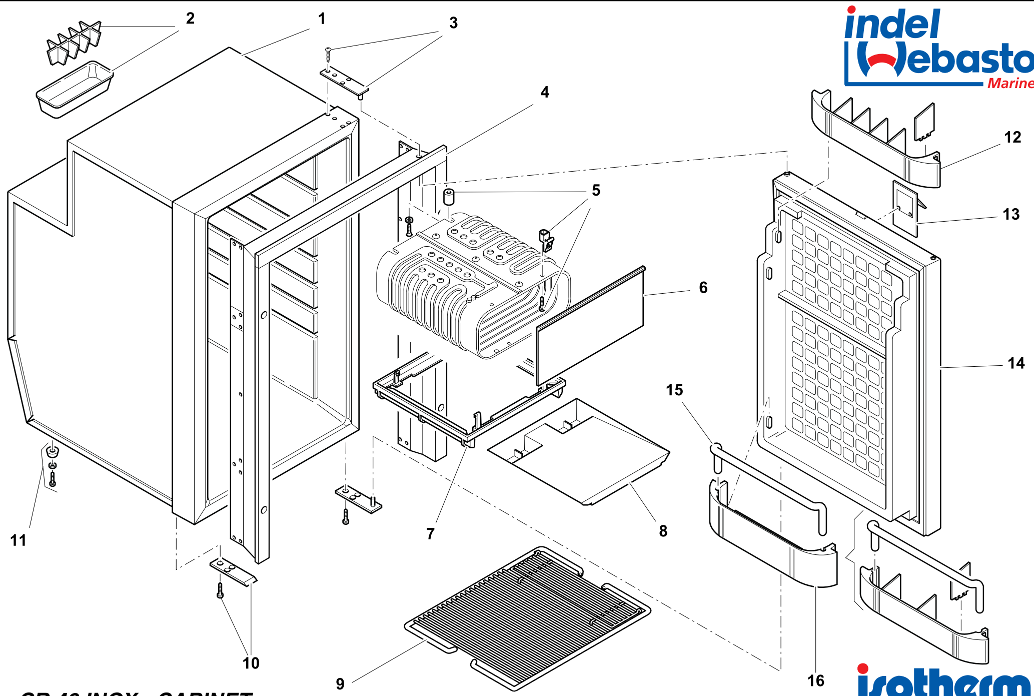
CR 49 INOX - CABINET
